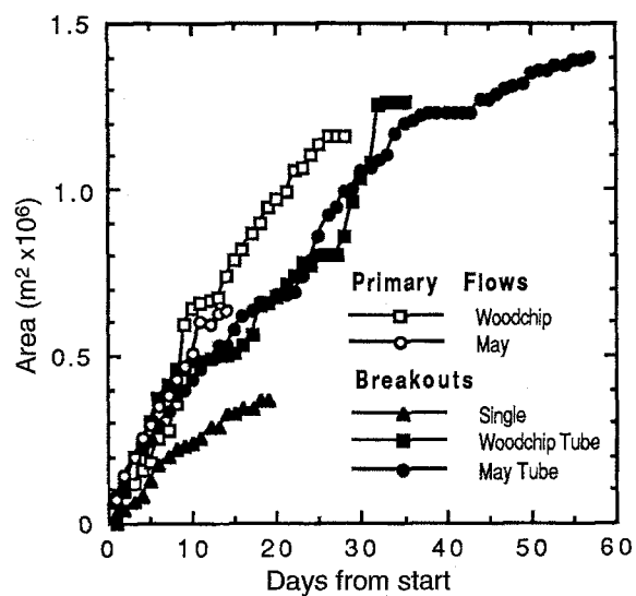
Fig. 3. Cumulative areas covered by May and Woodchip primary flows and by breakouts from tubes formed within those flows. A single breakout from the May tube is shown for comparison
