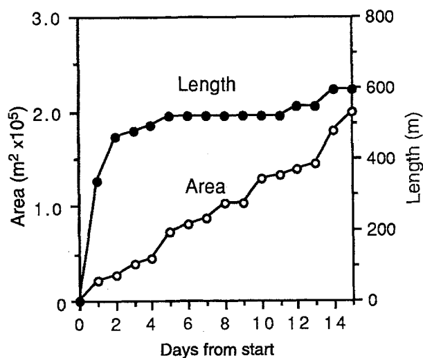
Fig. 4. Growth of a single breakout in length and area
