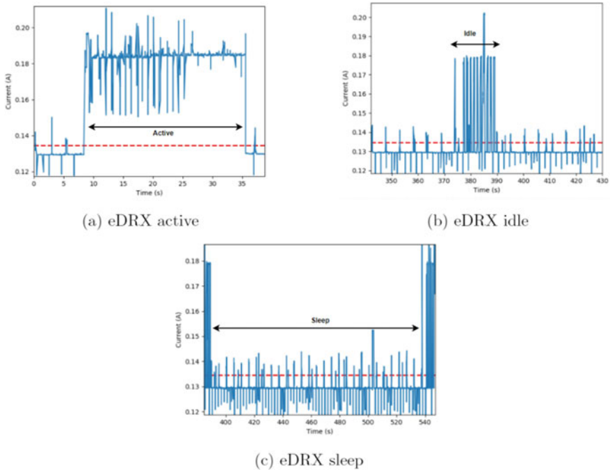
Fig. 13.8 eDRX active, idle, and sleep cycles
