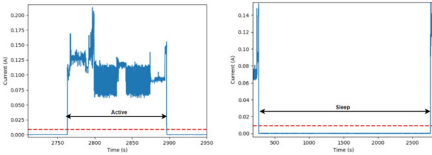
Fig. 13.6 PSM active and sleep cycles
