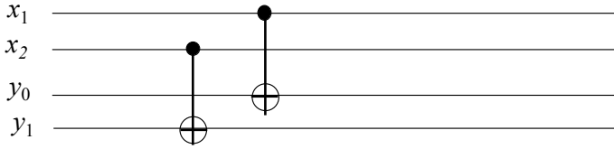
Fig. 6 Quantum circuit for N = 15 in Politi (2009)
