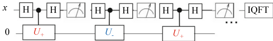
Fig. 8 Quantum circuit for N = 21 in Martin-Lopez et al. (2012)
