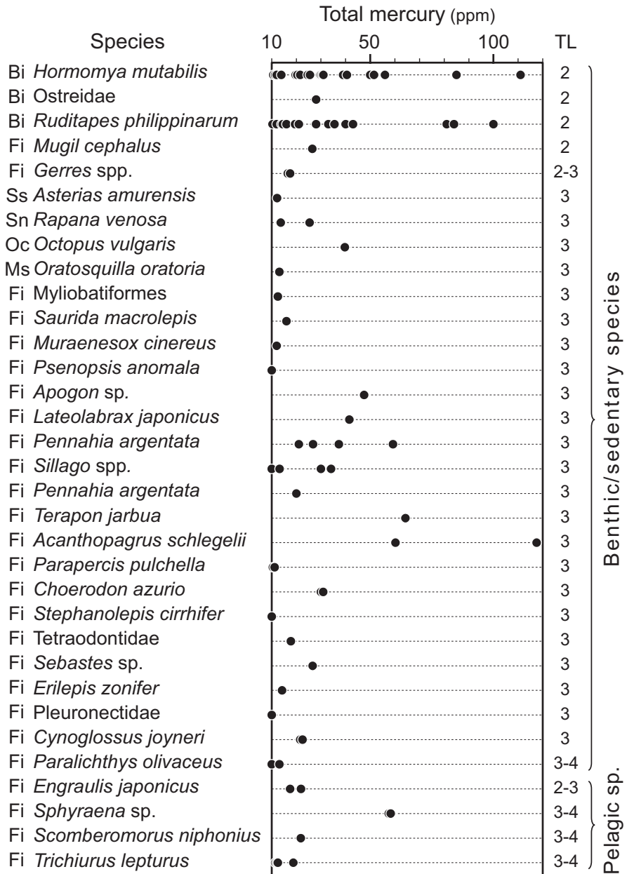
Fig. 2.11 Aquatic organisms showing high concentrations of total mercury (>10 ppm = \mu\text{g g}^{-1} dry wt) collected from Minamata Bay and the Shiranui Sea during the period from 1958 to 1966. Values which were shown in terms of wet weight in original papers were converted by multiplying 2.5 for fish or 5.0 for other animals. Abbreviations of animal groups are Sn = snail, Bi = bivalve, Oc = octopus, Ms = mantis shrimp, Ss = sea star, and Fi = fish. TL means the trophic level (suspension feeders and herbivores belong to TL 2, omnivores belong to TL 2-3, carnivores digesting invertebrates and small-sized fish belong to TL 3, and piscivores belong to TL 4) (Data source: Fishery Research Institute 1960; Kitamura et al. 1960b; Chisso Co. 1961; Kumamoto University 1961; Seikai Regional Fisheries Research Laboratory 1964; Irukayama et al. 1967b, 1972; and unpublished data of Chisso Co. after Nishimura and Okamoto 2001)
