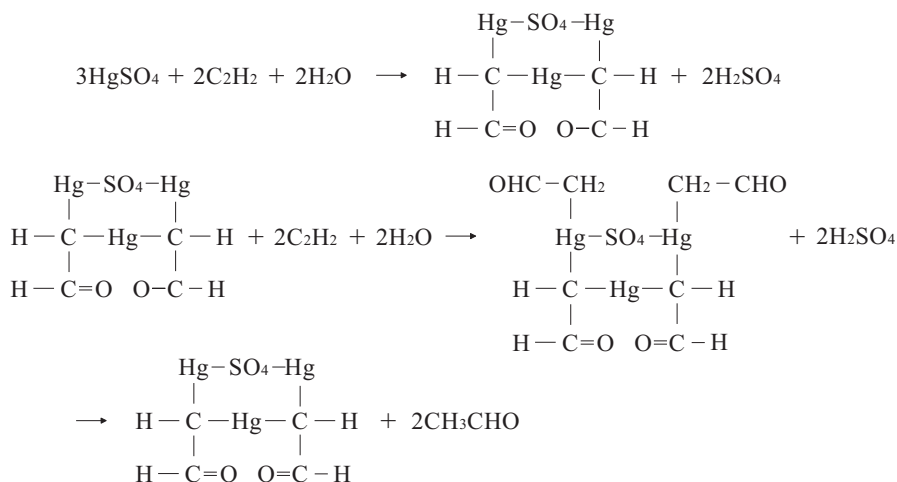
Fig. 2.16 Empirical chemical formulae in the acetaldehyde production shown by Vogt and Nieuwland (1921). Vogt and Nieuwland (1921) indicated that the catalytic mercury compounds being organic were readily hydrolyzed, resulting in the production of acetaldehyde
