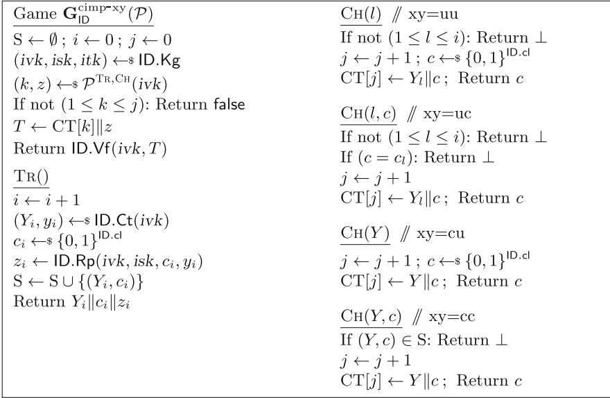
Fig. 4. Games defining security of identification scheme ID against constrained impersonation under passive attack.
