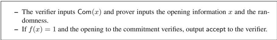
Fig. 2. The ideal functionality \mathcal{F}_{\text{Com},f}
