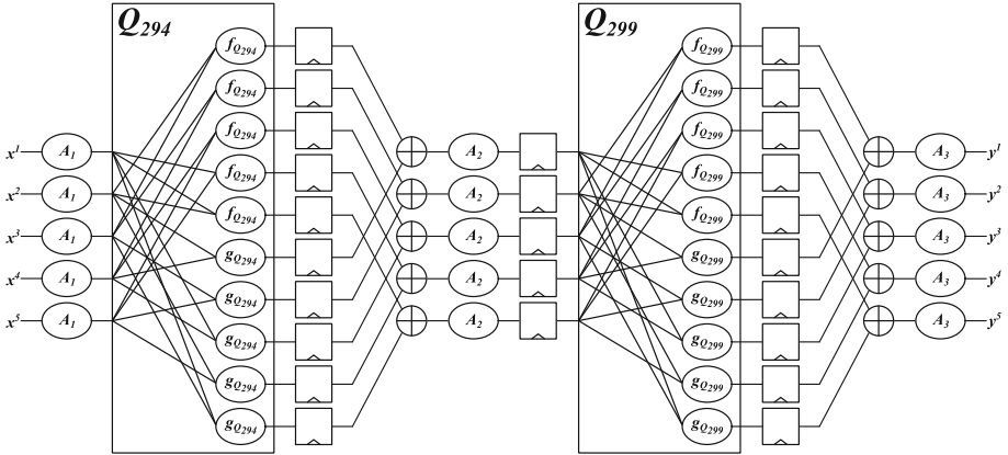
Fig. 4. A second-order TI of the PRESENT Sbox: S(x) = y
