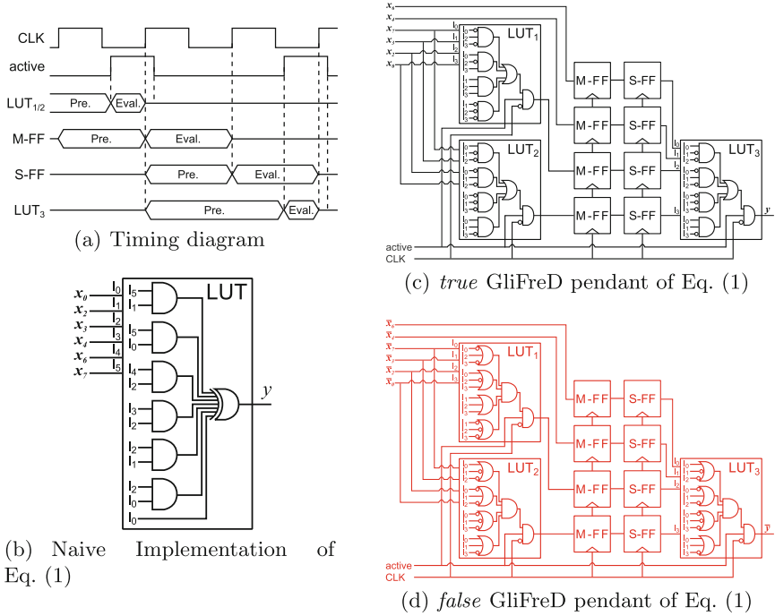
Fig. 1. An exemplary function implemented in a standard 6-to-1 LUT architecture and its GliFreD representation including the timing diagram
