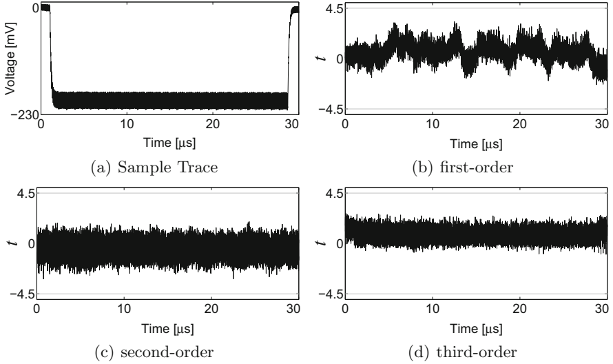
Fig. 10. PRESENT-1st-G profile, sample trace and non-specific t -test results using 1,000,000,000 traces
