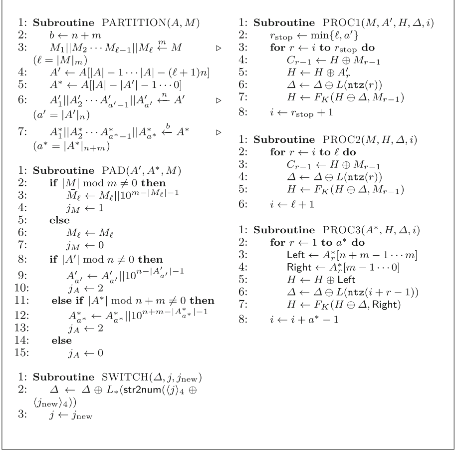
Fig. 3. The subroutines used in the encryption algorithm of p-OMD[ F, \tau ] (Fig. 2)
