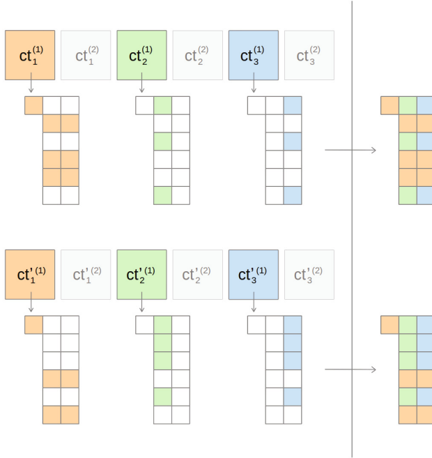
Fig. 3. The matrices of two 1SK-MIFE ciphertexts, ct = (ct_1^{(1)}, ct_2^{(1)}, ct_3^{(1)}) and ct' = (ct'_1{}^{(1)}, ct'_2{}^{(1)}, ct'_3{}^{(1)}) (both encrypted to slot 1), with the index set of each matrix depicted below it. Since the index sets are defined by two different elements of the same exclusive partition family, the adversary cannot “mix and match” elements from the two ciphertexts.
