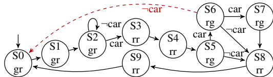
Fig. 9. Traffic light implementation
