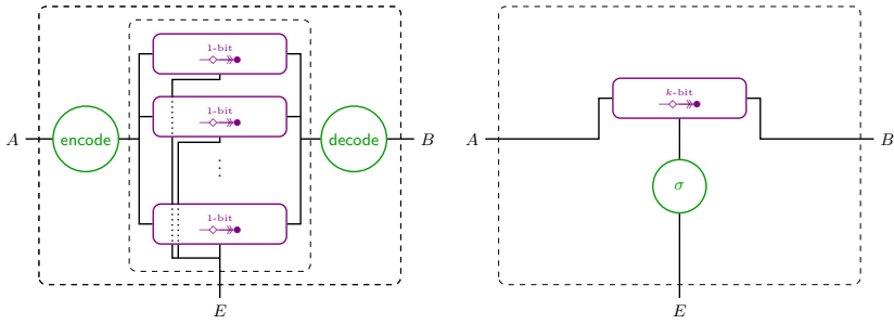
Fig. 5. Left: The assumed resource [\text{1-bit}]^n with protocol converters encode and decode attached to interfaces A and B , denoted \text{encode}^A \text{decode}^B [\text{1-bit}]^n . Right: The constructed resource [\text{k-bit}] with simulator \sigma attached to the E -interface, denoted \sigma^E [\text{k-bit}] . In particular, \sigma must simulate the E -interfaces of [\text{1-bit}]^n . The protocol is secure if the two systems are indistinguishable.
