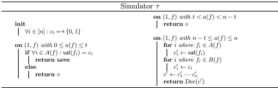
Fig. 9. The simulator \tau
