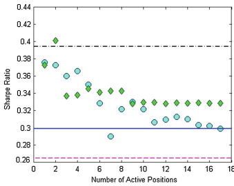
Fig. 11. Out-of-sample performance for FF17 measured by the Sharpe ratio over all the out-of-sample periods. See the caption of Fig. 10 for an explanation of the various symbols and lines.
