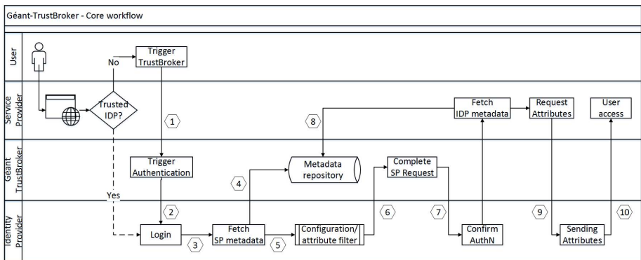
Fig. 1. GNTB's core workflow
