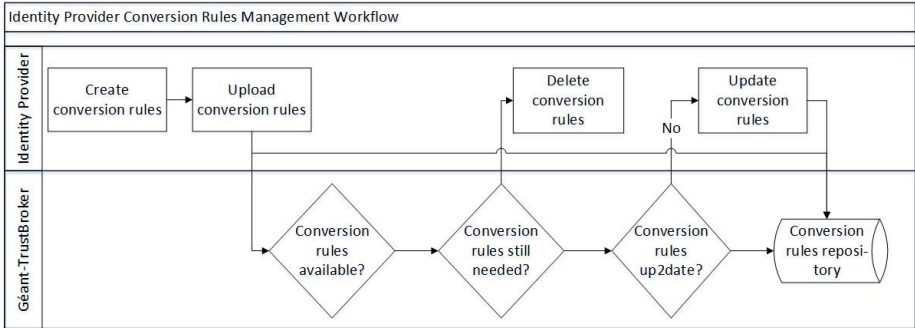
Fig. 4. Géant-TrustBroker workflow for conversion rules
