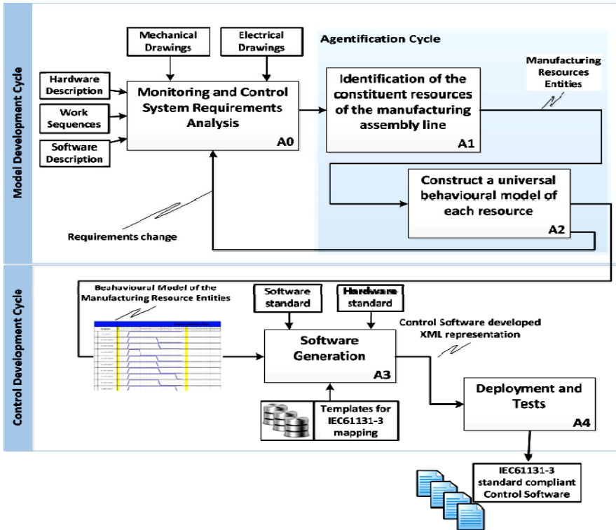
Fig. 2. Conceptual model of the Proposed Methodology
