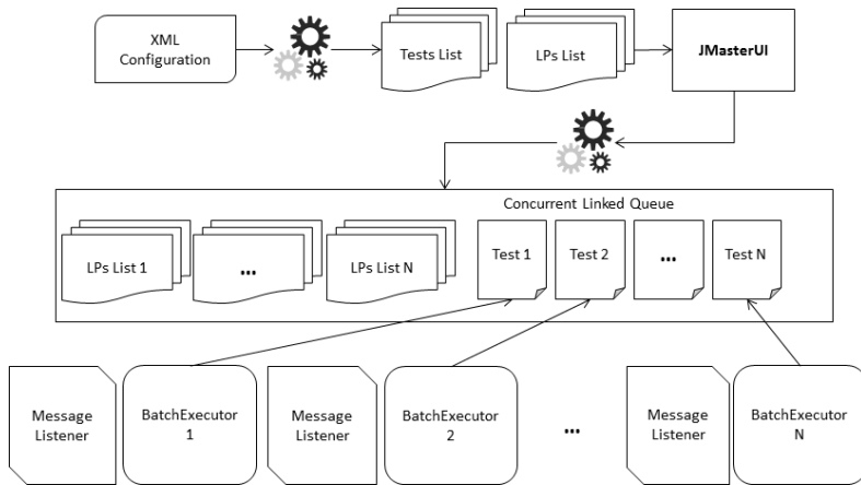
Fig. 5. Batch execution
