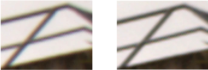
Fig. 1. Cropped and zoomed-in image from camera Canon EOS 40D, before (left) and after (right) chromatic aberration correction by our method. Notice the attenuated color fringes at edges between left and right images.
