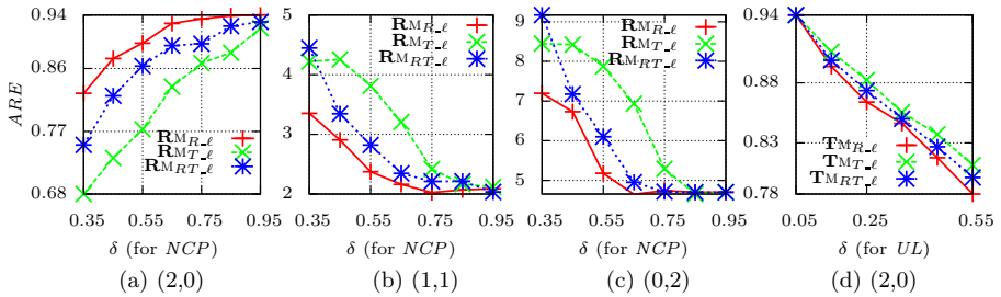
Fig. 5. ARE for queries involving (x, y) relational values and items. Figs. (a)-(c) are for INFORMS ( RM -BOUND); Fig. (d) is for INFORMS ( Tum -BOUND).
