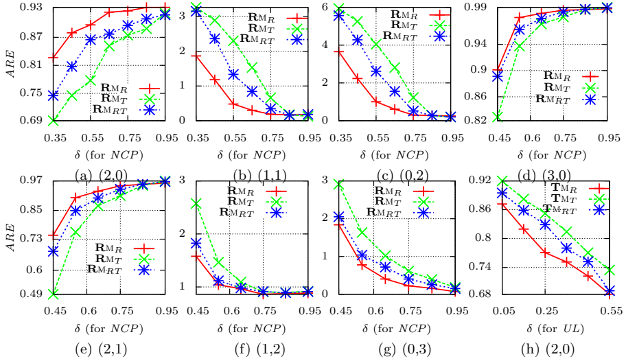
Fig. 4. ARE for queries involving (x, y) relational values and items. Figs. (a)-(c) are for INFORMS; (d)-(g) for YOUTUBE ( RM -BOUND). Fig. (h) is for INFORMS ( Tum -BOUND).
