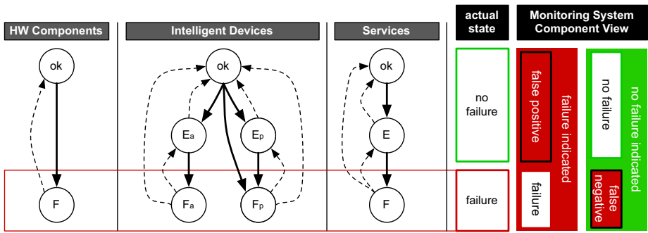
Fig. 2. State machines for components and services and the perception of their state in the monitoring system
