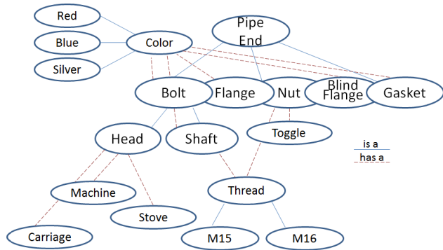
Fig. 10. A Simple Pipe End Ontology
