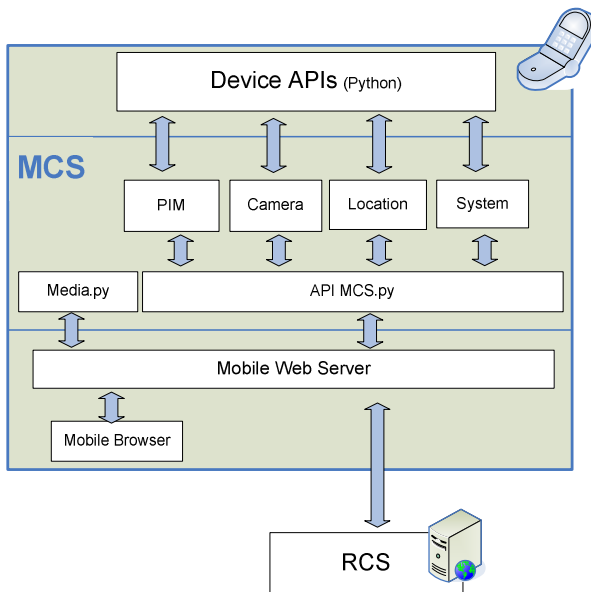
Fig. 3. MCS architecture
