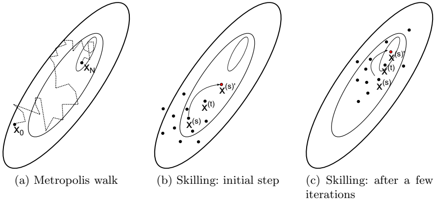
Fig. 3. Markov-Chain Monte-Carlo
