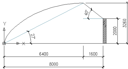
Fig. 1. Sectional view of the solar greenhouse
