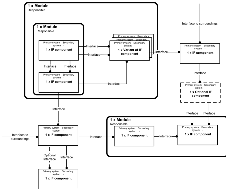
Fig. 4. Symbolic representation of a generic interface diagram
