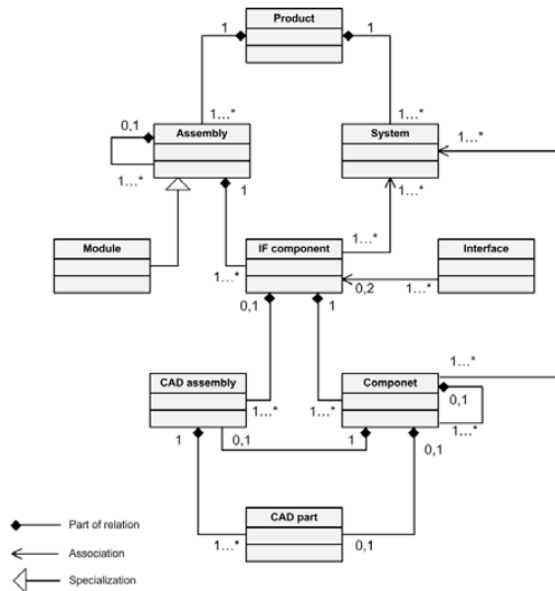
Fig. 8. Entity relation model of the structures loaded into a PLM system
