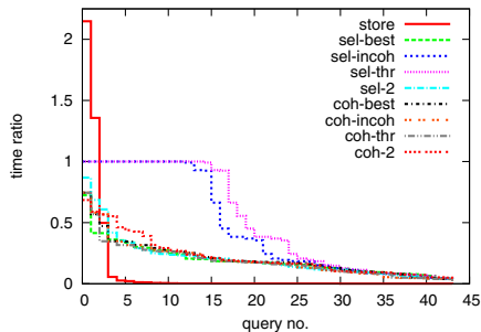
Fig. 9. Queries ordered by time for different order and split strategies
