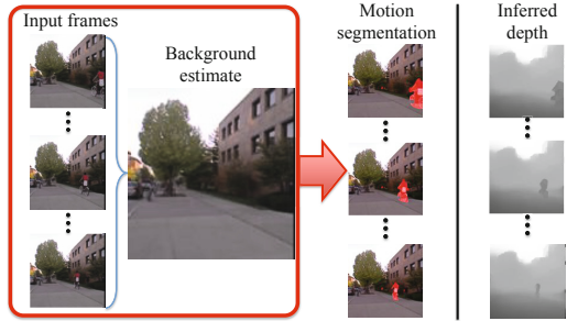
Fig. 5. We apply median filtering on the stabilized images to extract the background image. A pixel is deemed to be in motion if there is sufficient relative difference from the background image.
