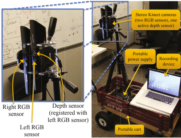
Fig. 6. Our stereo-RGBD collection rig consists of two side-by-side Microsoft Kinects. The rig is mobile through the use of an uninterruptible power supply, laptop, and rolling mount.
