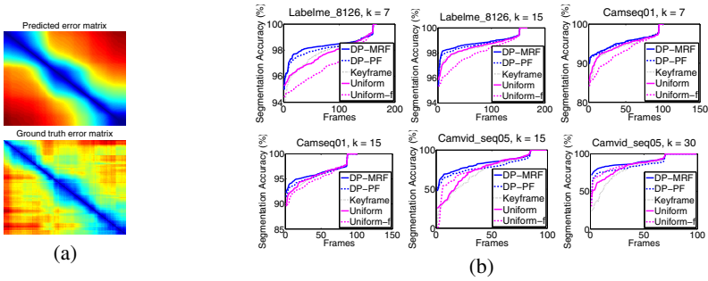
Fig. 5. (a) Comparison of ground truth label propagation error with the error predicted by our model ( C ) for Labelme. Our error predictions follow the actual errors fairly closely. (b) Each method’s accuracy plotted for all frames, for two values of k per sequence. Accuracy values are sorted from high to low per method for clarity. Our DP approaches (darker blue curves) have higher accuracy, esp. on frames far from labeled frames. Best viewed on pdf.
