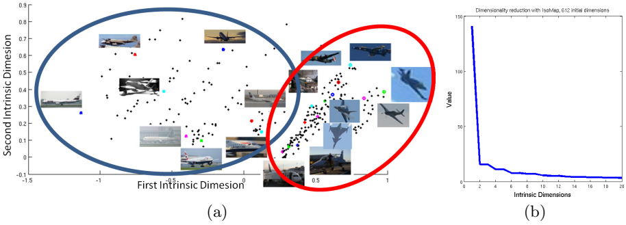
Fig. 1. (a) Visualization of the \chi^2 similarity metric using Isomap. The two ellipses show the clustering of the training instances of the 'Aeroplane' category of PASCAL VOC 2007. As can be seen the clustering splits the data into very meaningful groups. (b) The visualization is accurate since the first two dimensions cover most of the variation.
