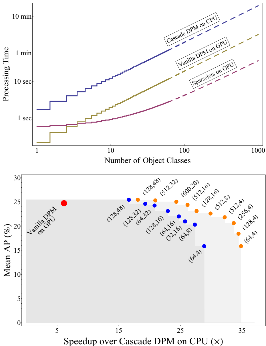
Fig. 6. Top: Comparison of cascade algorithm on CPU vs. vanilla DPM on GPU vs. sparselets accelerated DPM on GPU as number of object classes grows. Sparselet accelerated DPM on GPU offers approximately 35 times faster compared to the cascade implementation on CPU. Frame size used in this experiment was 640 \times 480 . Bottom: Speedup vs. Mean AP. Blue dots are for “online” results measuring end-to-end time. Orange dots are for “post-hoc” case. The tuple in parenthesis denote (K, \epsilon) .
