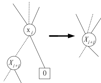
Fig. 2. pD-deletion rule
