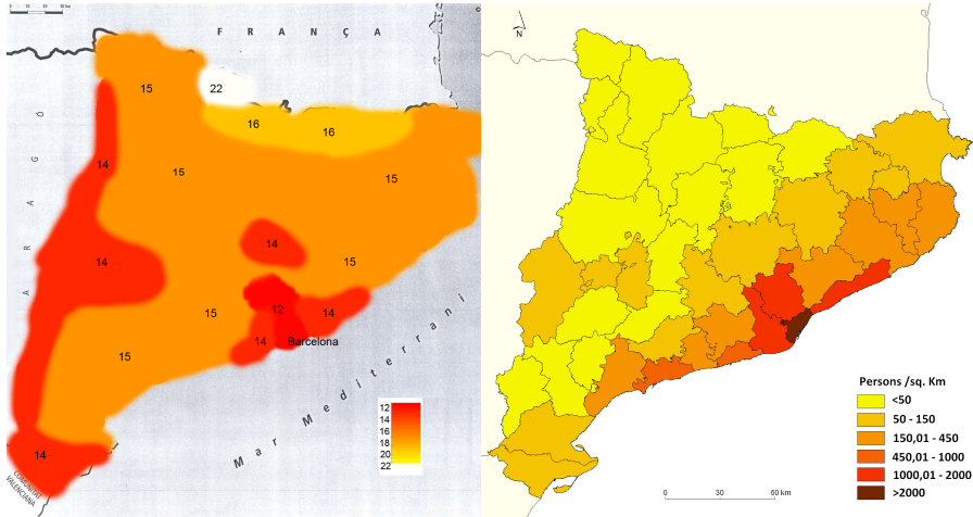
Fig. 1. 2015 Catalanian UHF channel availability map made by the authors ( left map ) and Catalan density map ( right map ), white or yellow areas are for density below 50 inhabitants per square km and black or red areas for densities higher than 1000 inhabitants per square km
