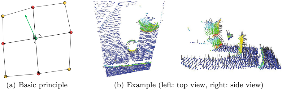
Fig. 1. Principle of fast normal computation using integral images (a). Two vectors tangential to the surface at the desired position are computed using the red points. The local surface normal is computed by applying the cross product to them. A typical result of an acquired point cloud with surface normals is shown in (b).
