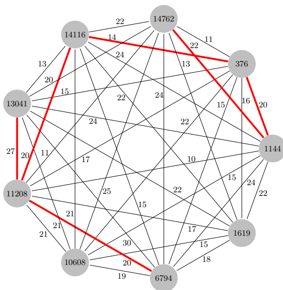
Fig. 6. Connected component consisting of nine vertices, corresponding to primes p_{376} , p_{1144} , \dots , p_{14762} (all 512-bit). With labels as in Figure 4, in total 687 X.509 certificates are involved. Six of those certificates have not expired yet, use SHA1 as hash function (as opposed to MD5), and have “CA=false”; the red edges correspond to the RSA moduli contained in those six certificates.
