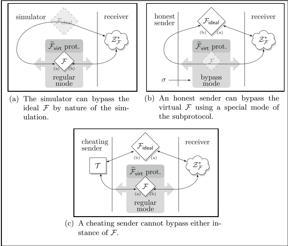
Fig. 2. Intuition behind the reveal phase of \Pi_{EqCom}^{\mathcal{F}} and its security properties
