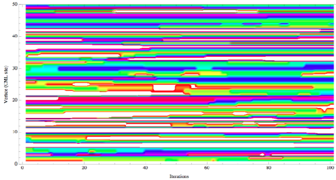
Fig. 3. Dynamics of the complex network visualized like CML system with edges deactivation by real number coefficient. Different colors including white one represent different vertices (sites) activation.
