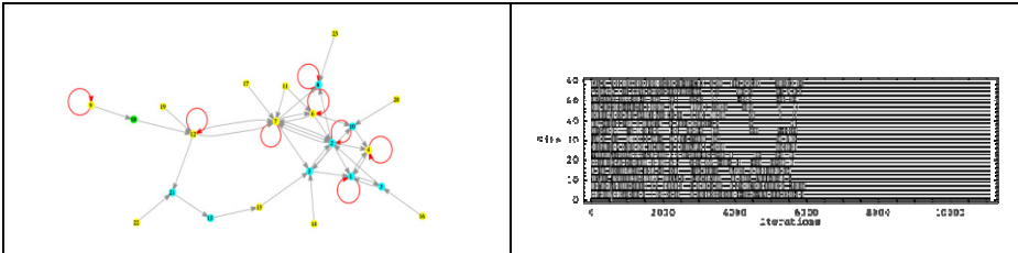
Fig. 1. Example: complex network with more vertices (left), typical CML behavior with chaotic and deterministic “windows”, after iteration 6000 it is due to the control fully stabilized (right)
