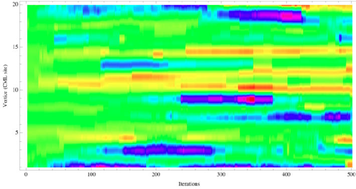
Fig. 2. CML of the network with 20 vertices in 500 iterations
