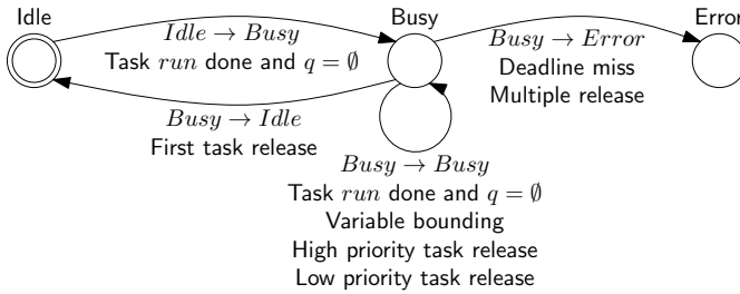
Fig. 5. A high level overview of the scheduler and queue encoding in timed automata
