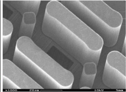
Fig. 3. SEM closeup of a 4x4 MDA chip (poly silicon layer 65μm thick)
