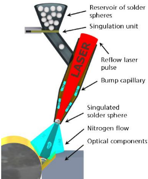
Fig. 6. Simplified schematics of the solder bumping bond head
