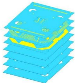
Fig. 5. Schematics of the LTCC carrier layer stack
