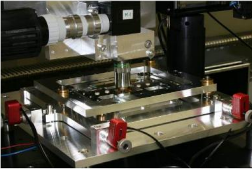
Fig. 8. Assembly device
