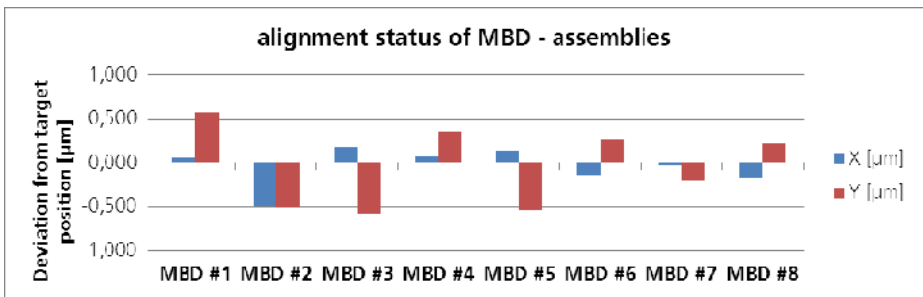
Fig. 12. Alignment status of MBD assemblies in x- and y-direction
