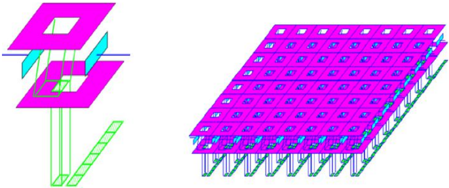
Fig. 1. Schematic comparison of VSB (left) and MSB (right) exposure principle
