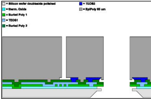
Fig. 2. Cross section of a poly silicon MDA
