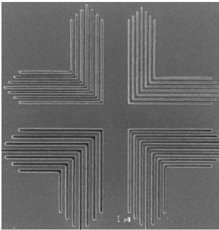
Fig. 13. Resist image of resolution test pattern (1:1 lines and spaces) exposed with the MSB 3050 test tool in HSQ resist on silicon wafer: lower left 40 nm, lower right 35 nm, upper left 30 nm, upper right 25 nm line width.
