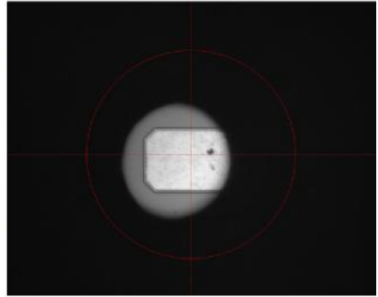
Fig. 9. MDA contact pad inside a via hole of the LTCC carrier
