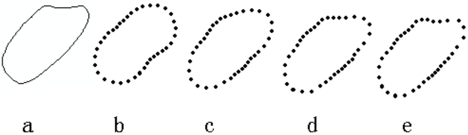
Fig. 5. Diagram showing restoration of the rice shape with different number of Fourier low-frequency components: (a) original image; (b) restoration with 3 components; (c) restoration with 5 components; (d) restoration with 7 components; and (e) restoration with 9 components
