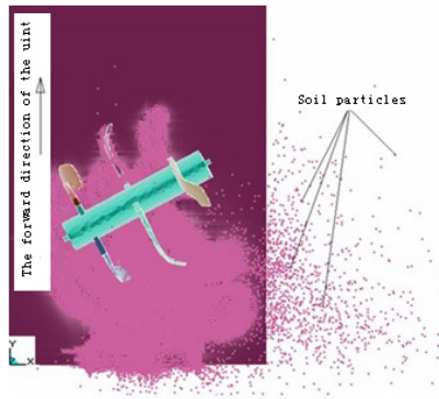
Fig. 13. Throwing Soil simulation of oblique rotary tilling
