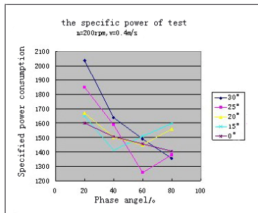
Fig. 9. The specific power of test
