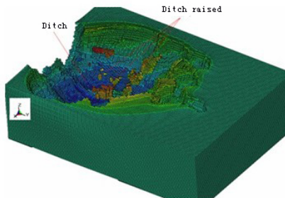
Fig. 14. Furrow bottom shape
