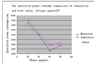
Fig. 11. The specified power consume comparison of simulation and test value, oblique angle=25°
