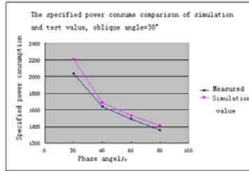
Fig. 10. The specified power consume comparison of simulation and test value, oblique angle=30°
