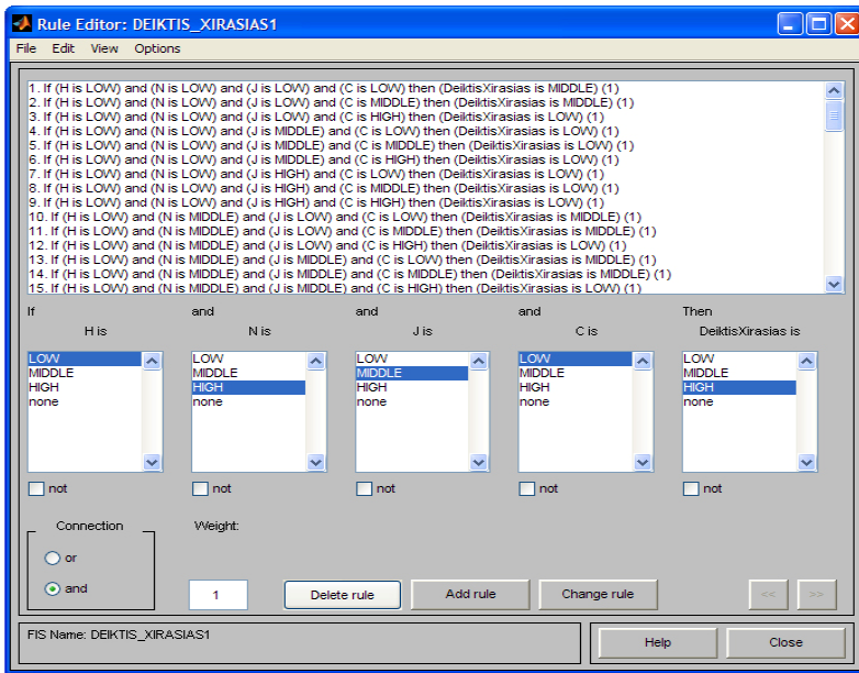
Fig. 2. Design of the fuzzy Ruleset in MATLAB
