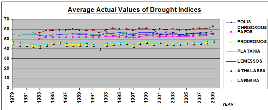
Fig. 6. AAVDI risk indices values for the period 1979-2009
