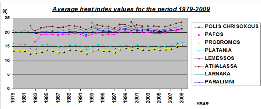
Fig. 8. Average heat index values for the period 1979-2009
