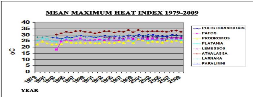
Fig. 7. Mean Maximum Heat Index 1979-2009
