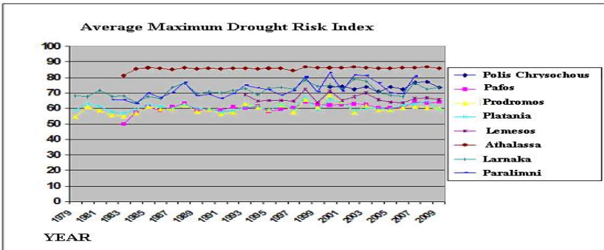
Fig. 4. Average Maximum Drought risk indices 1979-2009
