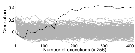
Fig. 6. Correlation evolution vs. Number of executions for AES_TI (130nm)
