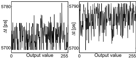
Fig. 14. Timing characteristics T^o of S-box instances no. (left) 2 and (right) 3 of AES_MDPL (65nm)
