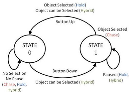
Fig. 2. State Transition Diagram for methods of interaction
