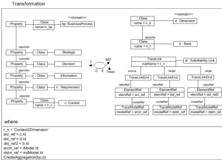
Fig. 6. QVT transformation for deriving a context into a dimension with its associated trace
