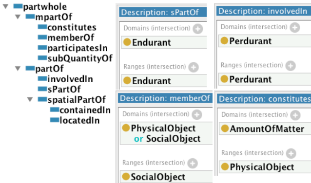
Fig. 2. The OWLized version of the taxonomy of part-whole relations [14] (left) with screenshots of domain and range restrictions of four object properties (right)
