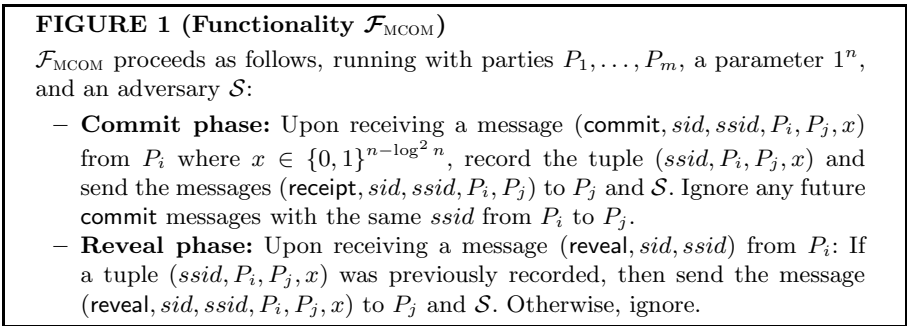
Fig. 1. The ideal commitment functionality
