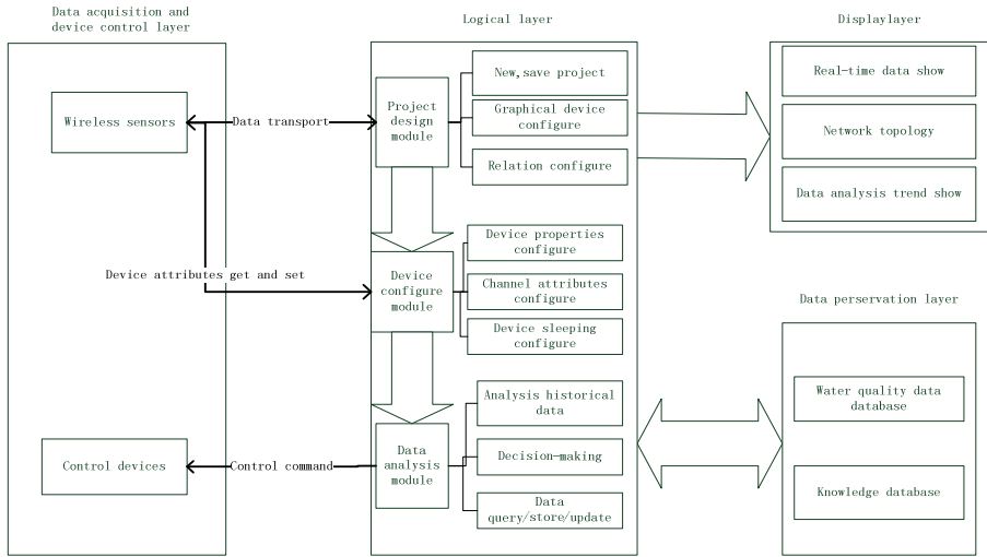
Fig. 3. Software architecture
