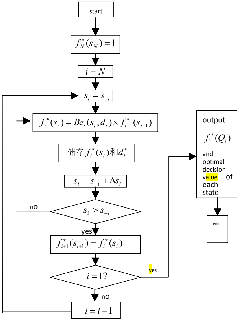
Fig. 2. Program of reverse algorithm of dynamic planning
