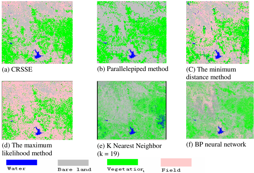
Fig. 3. Classification Results
