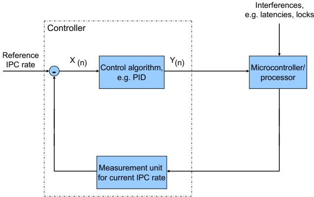
Fig. 3. Use of a controller to stabilize the throughput
