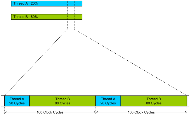
Fig. 2. Example for GP scheduling
