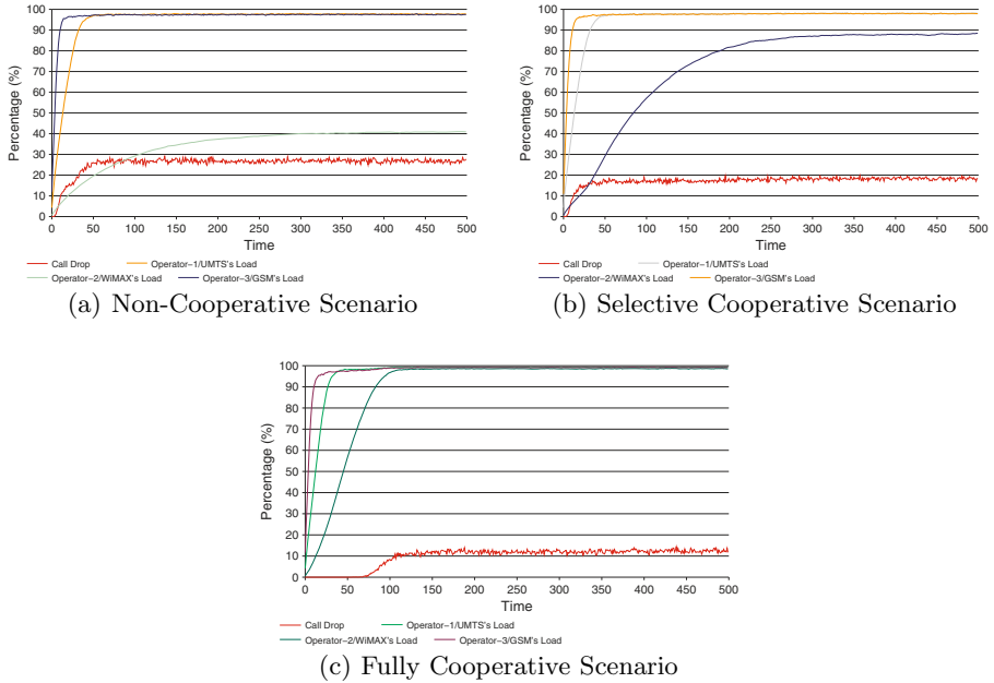
Fig. 1. Resource utilization and call blocking rate for different cooperation levels
