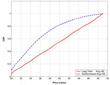
(b) CDF curve of handovers
