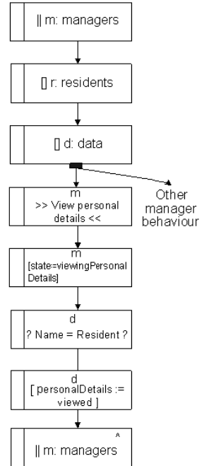
Fig. 5. Manager thread
